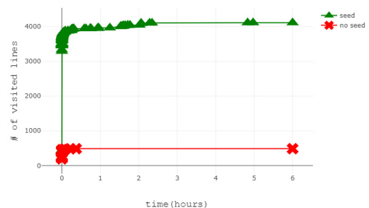
Fig. 3. Line coverage comparison between when seeds are given and when not given
